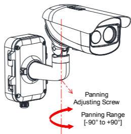
Figure 2-25 P-Axis Adjustment
