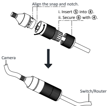
Figure 2-26 Water-proof Accessory Installation
