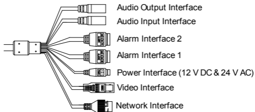
Figure 1-8 Type III Camera Cables
