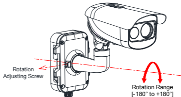
Figure 2-23 R-Axis Adjustment
