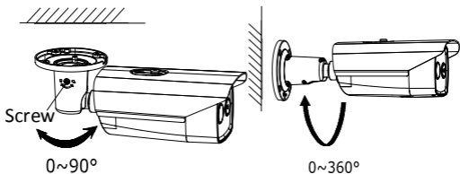
Figure 2-17 2-axis Adjustment
