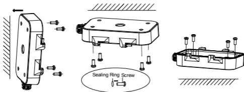
Figure 2-21 Installing Junction Box Base
