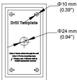
Figure 2-20 Drill Template
