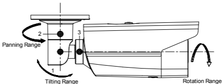
Figure 2-16 3-Axis Adjustment
