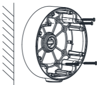
Figure 2-2 Drill the Holes and Fix the Junction Box
