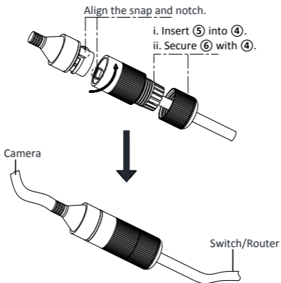
Figure 2-8 Waterproof Accessory Installation
