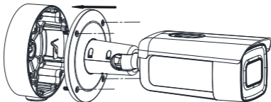
Figure 2-4 Install the Camera
