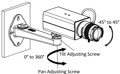
Figure 2-7 Adjusting the Surveillance Angle
