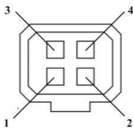
Figure 1-4 Auto-iris Interface
