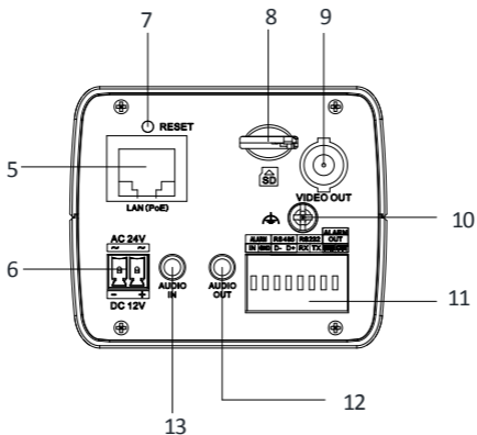
Figure 1-3 Interfaces on the Rear Panel
