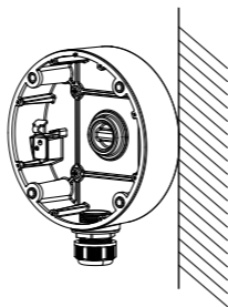
Figure 2-8 Secure the Junction Box's Body on the Ceiling/Wall
