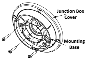
Figure 2-7 Fix screws on the junction box's Cover
