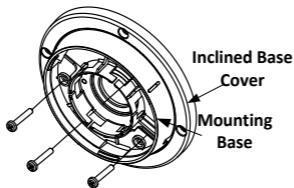
Figure 2-10 Fix Camera's Mounting Base
