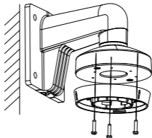
Figure 2-13 Install the Mounting Base on the Wall Mounting Bracket
