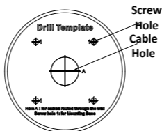
Figure 2-9 Drill Template
