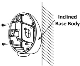
Figure 2-11 Fix the Inclined Base's boy on Ceiling/Wall
