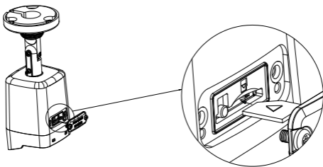
Figure 2-1 Unscrew the Cover and Insert Memory Card
